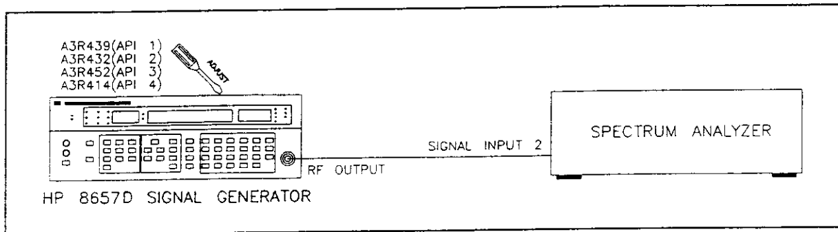
Figure 5-15. API 1, 2, 3 and 4 Adjustment Setup
