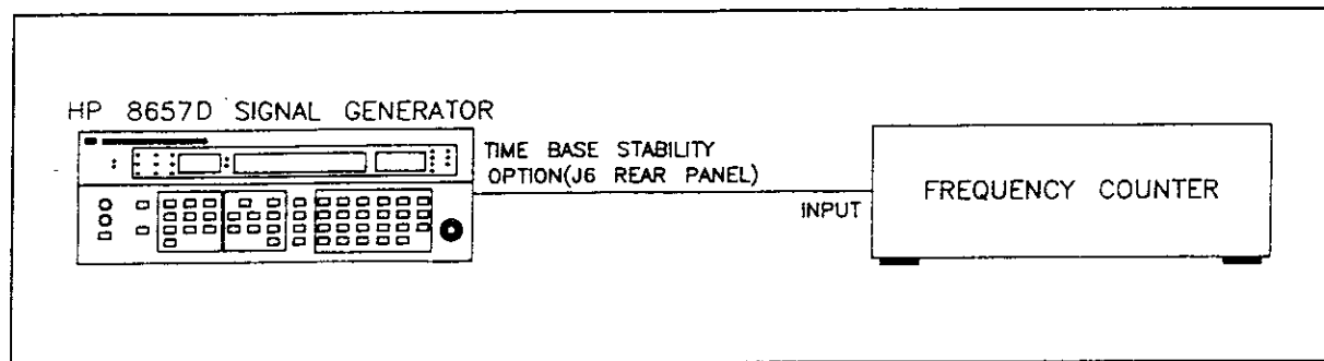
Figure 5-23. 10 MHz Reference Oscillator Frequency Adjustment Setup
