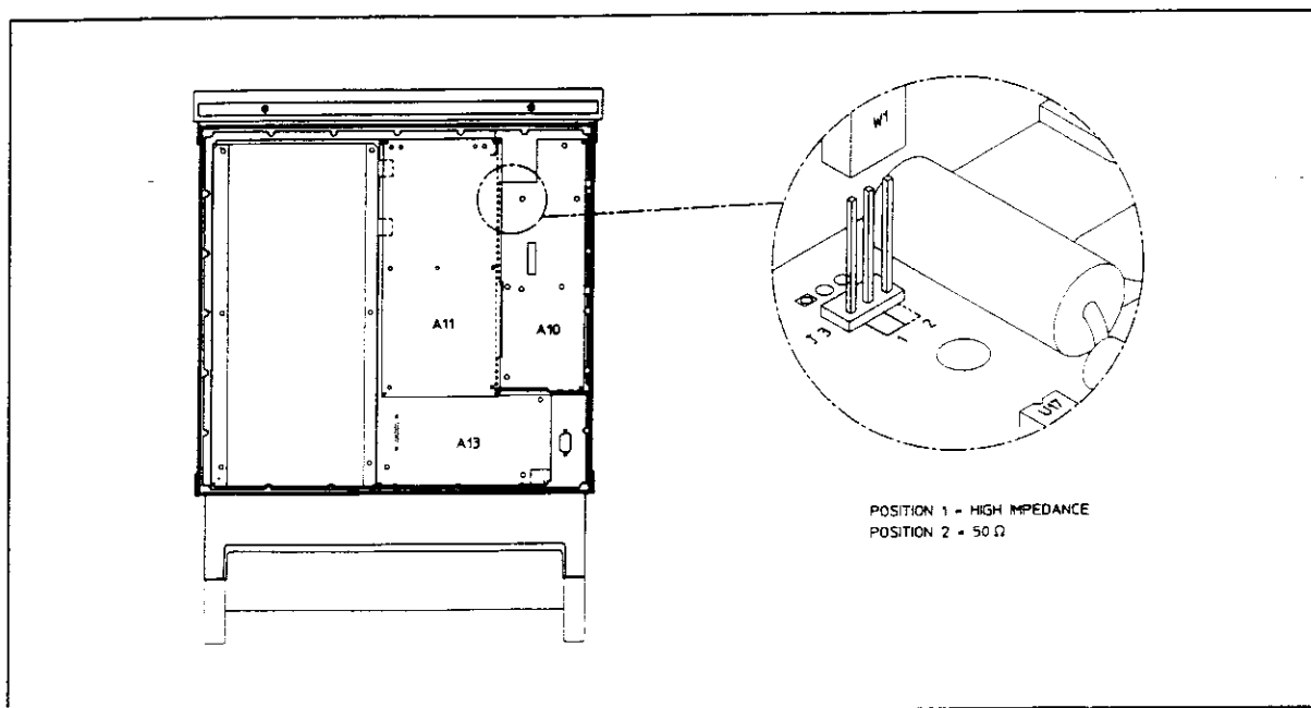
Figure 2-5. Pulse Modulation Input Impedance Selection
