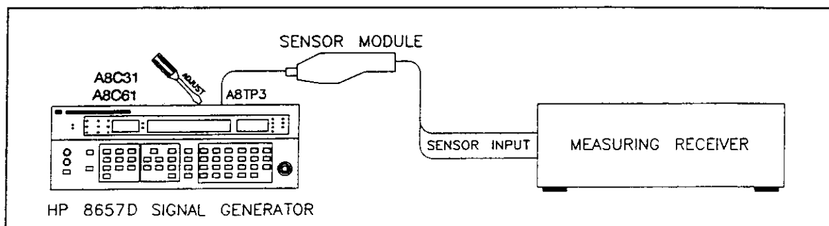
Figure 5-8. 200/400 MHz Bandpass Filter Adjustment Setup
