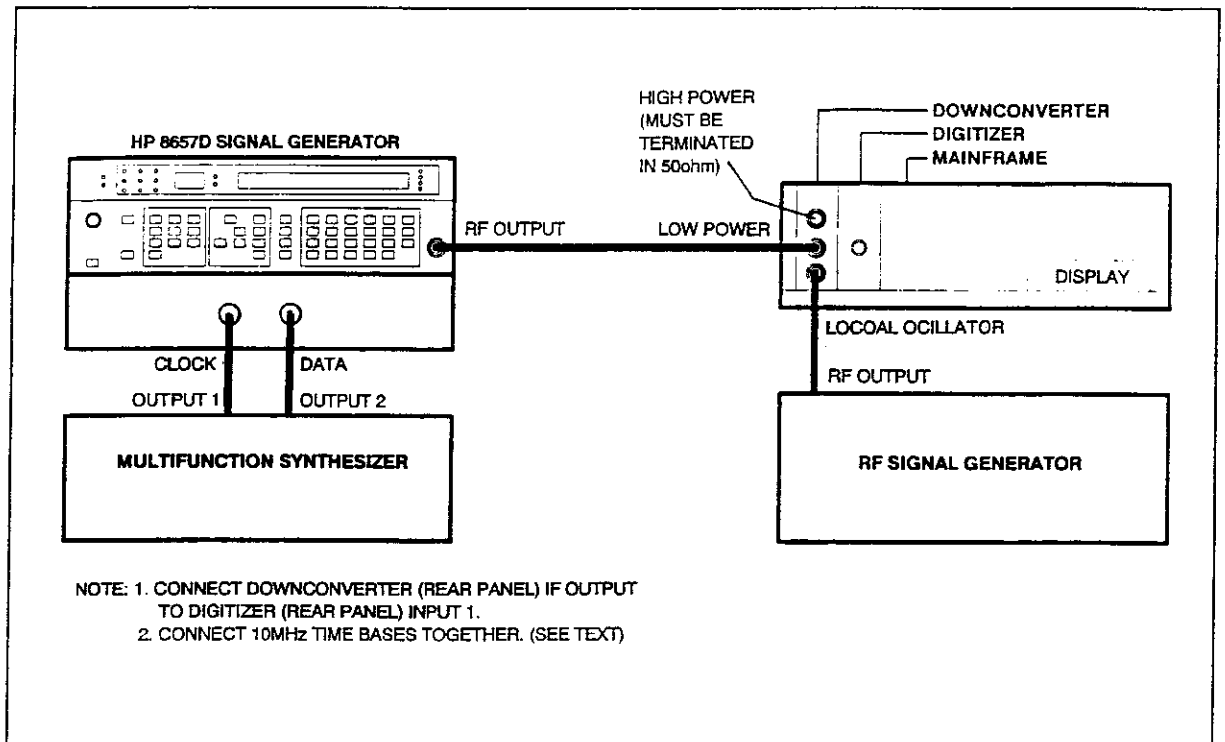
Figure 4-15. \pi/4 DQPSK Modulation Test Setup
