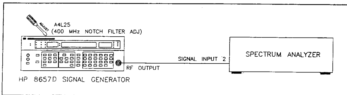
Figure 5-11. 400 MHz Notch Filter Adjustment Setup.
