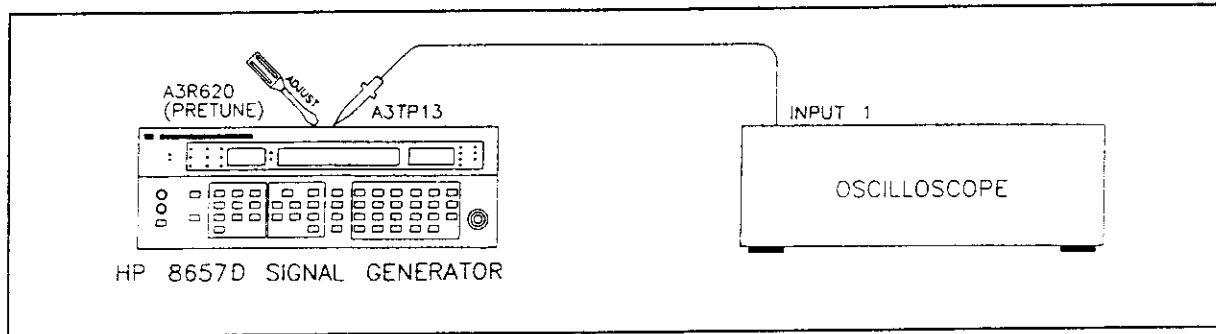
Figure 5-14a. FM Calibration Pretune Adjustment Setup
